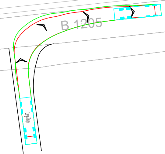
Tipper Vehicle Exiting Site Scale 1:500
