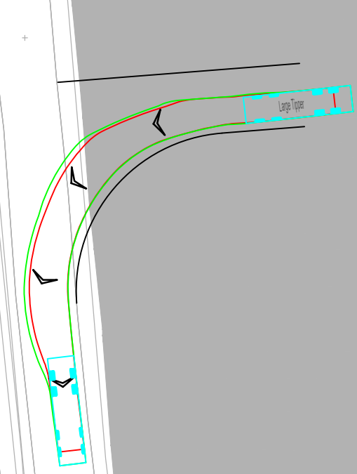
Tipper Vehicle Exiting Site Scale 1:500
